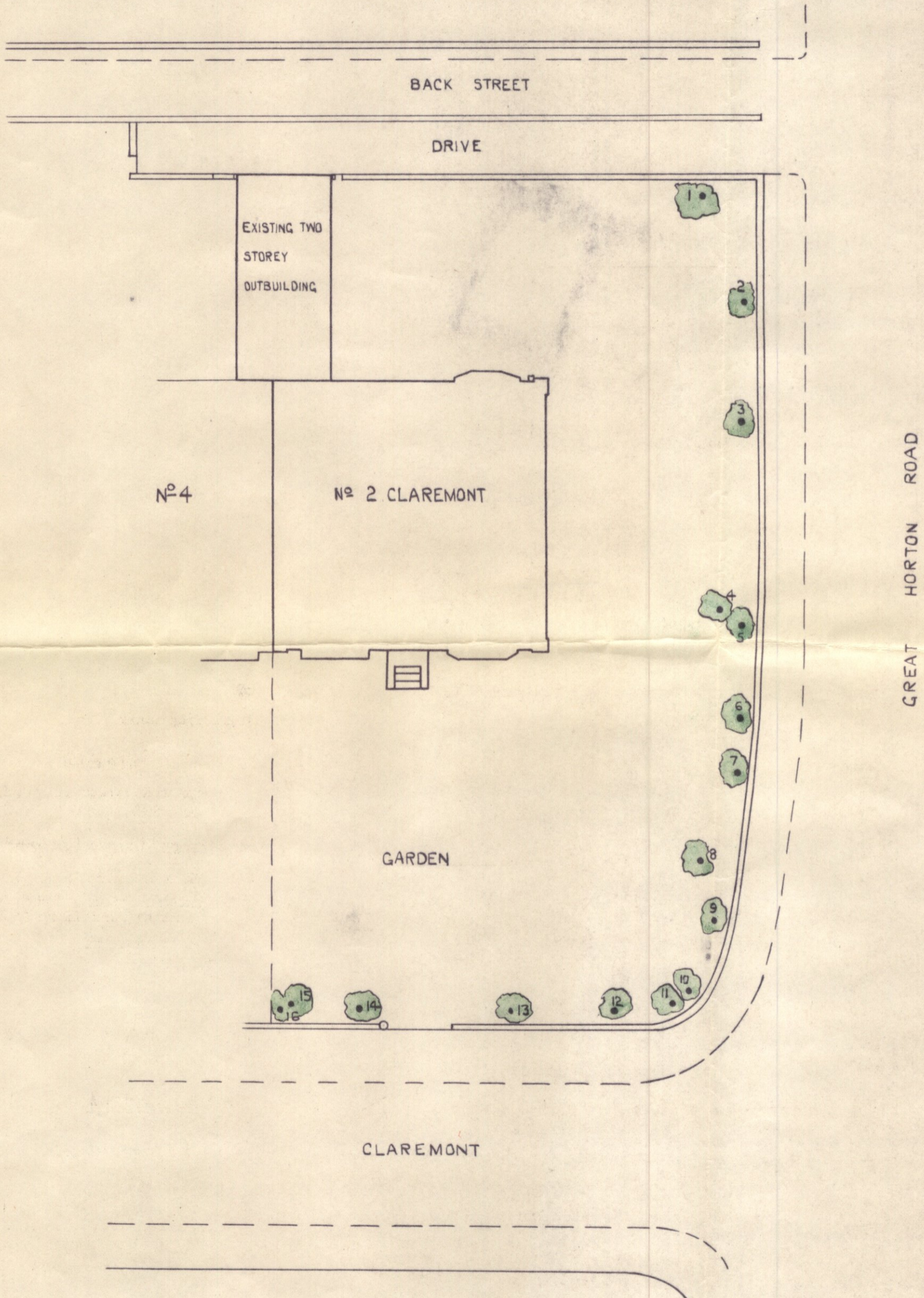
SITE PLAN SCALE 16'-0" TO 1"
